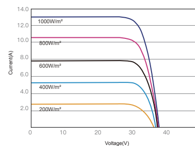
I-V CURVES OF PV MODULE(500W)
